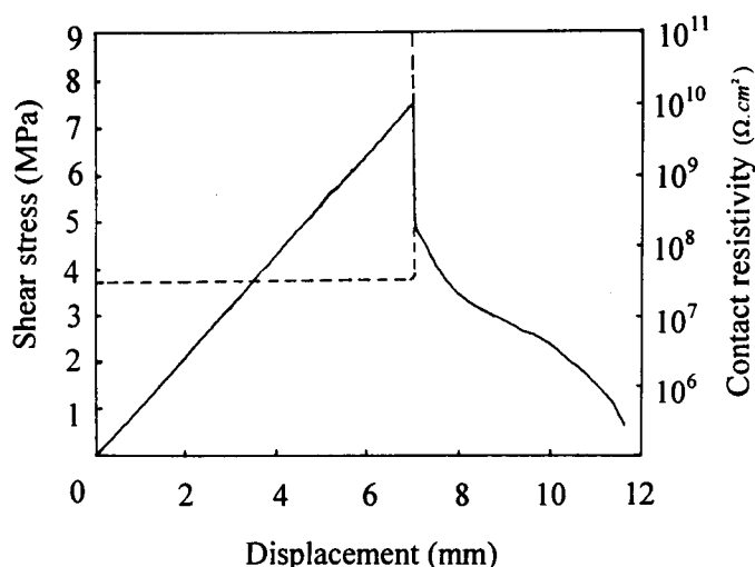
Fig. 2 Plots of shear stress vs. displacement (solid curve) and of contact electrical resistivity vs. displacement (dashed curve) simultaneously obtained during pull-out testing of steel rebar from concrete at 28 days.
